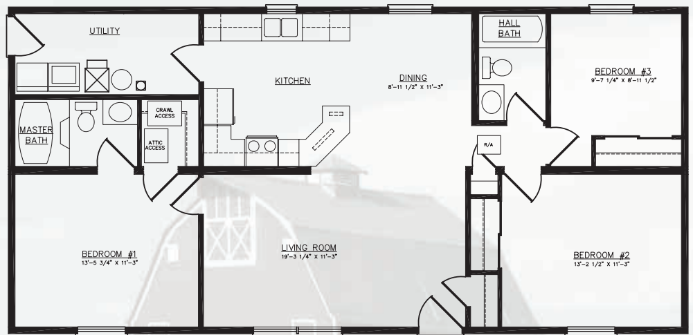
CRAWLSPACE PLAN
